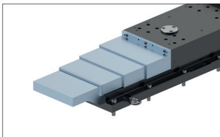
Telescopic protection
