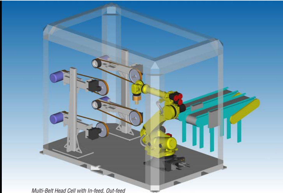
Multi-Belt Head Cell with In-feed, Out-feed
