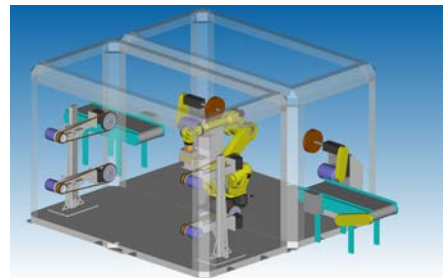
Belt and Wheel Head Cell
